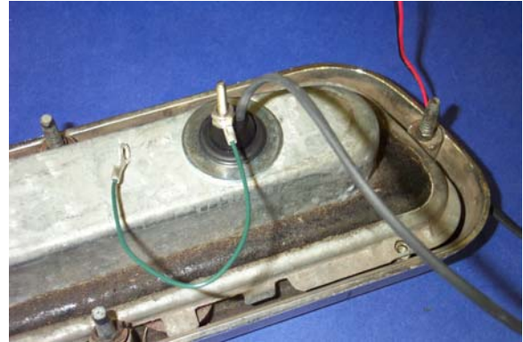
Install ground wire. Route wire to convenient screw location or cut ring terminal and splice to car's ground circuit. Very important!
