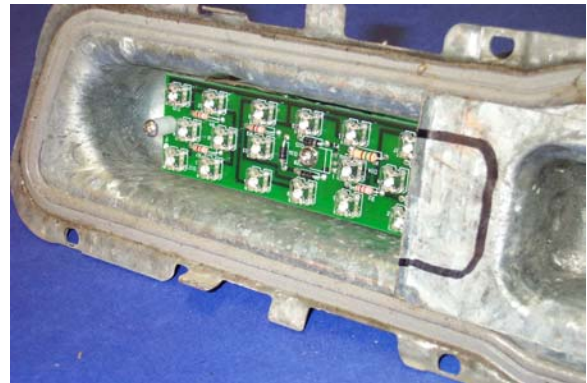
Optional: This area may be cut out to provide more light for the stoplights.
