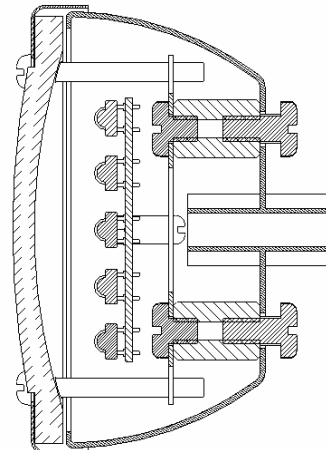
Top view cross-section showing completed assembly. '30-'32 housing shown. Stanchion not depicted.
